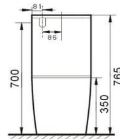
Frontal view
