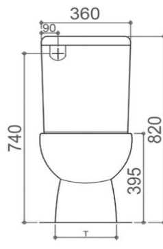
Frontal view
